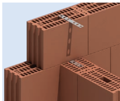
Ties for Internal Wall Junctions
