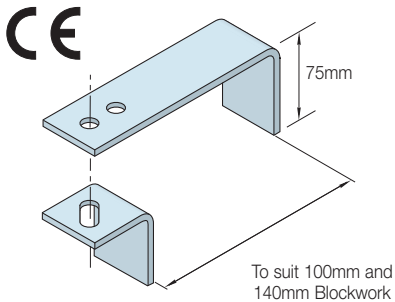
Ancon FHR Head Restraint - other sizes available
