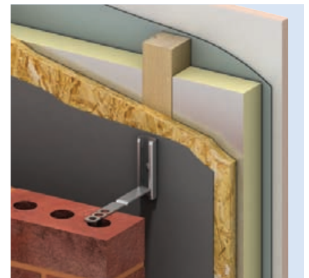
Ancon TFMT7 Timber Frame Movement Tie
