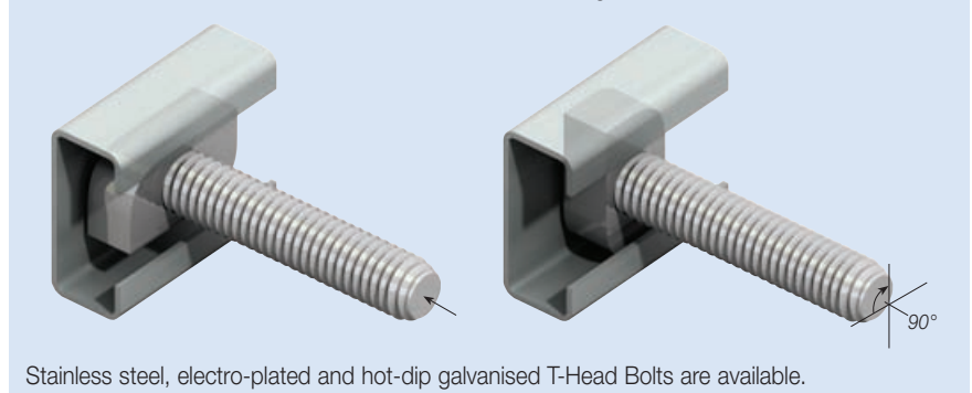
T-Head Bolts Inserted into Channel and Turned Through 90°
